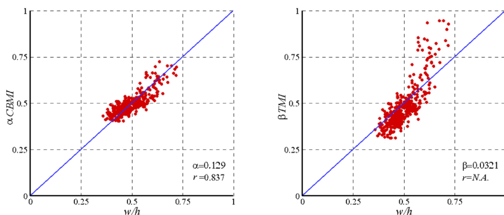
Fig. 2. (a, b) Waist-to-height ratio w/h versus \alpha \cdot \text{CBMI} (left, r = 0.837 ) and \beta \cdot \text{TMI} (right, r = \text{N.A.} ) for entire data set.
