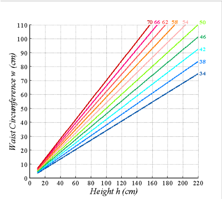
Fig. 3. Classification of anthropometric status levels according to 100-waist-to-height ratios. Interval between 42 and 50 normal levels with ideal average 46.
