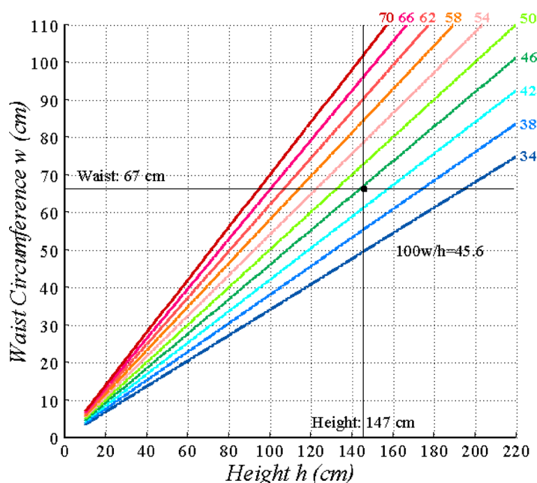
Fig. 5. A sample graphical assessment of anthropometric status level for a 10-year-old female: 147 cm height and 67 cm waist circumference. Assessed normal with 100 w/h = 45.6 , nearly equal to ideal normal 46.
