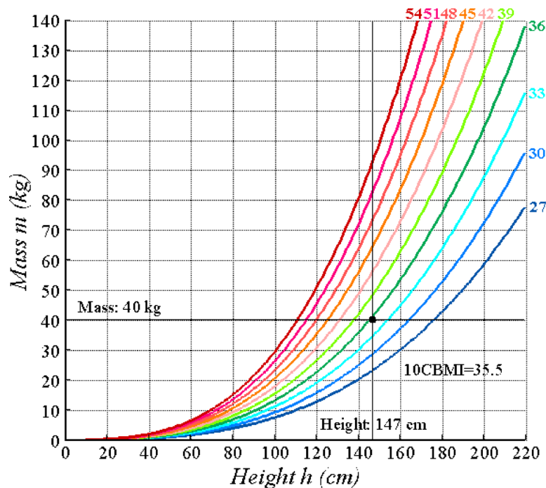
Fig. 6. A sample graphical assessment of anthropometric status level for a 10-year-old female: 40 kg mass, 147 cm height. Assessed normal with 10 CBMI=35.5 slightly less than ideal normal 36.
