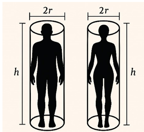
Fig. 1. Representation of human body as a circular cylinder with radius r and height h . Geometric measure of slowness or fullness of an object: Waist-to-height ratio w/h = \pi (2r/h) (width/height), where waist circumference w = 2\pi r .
