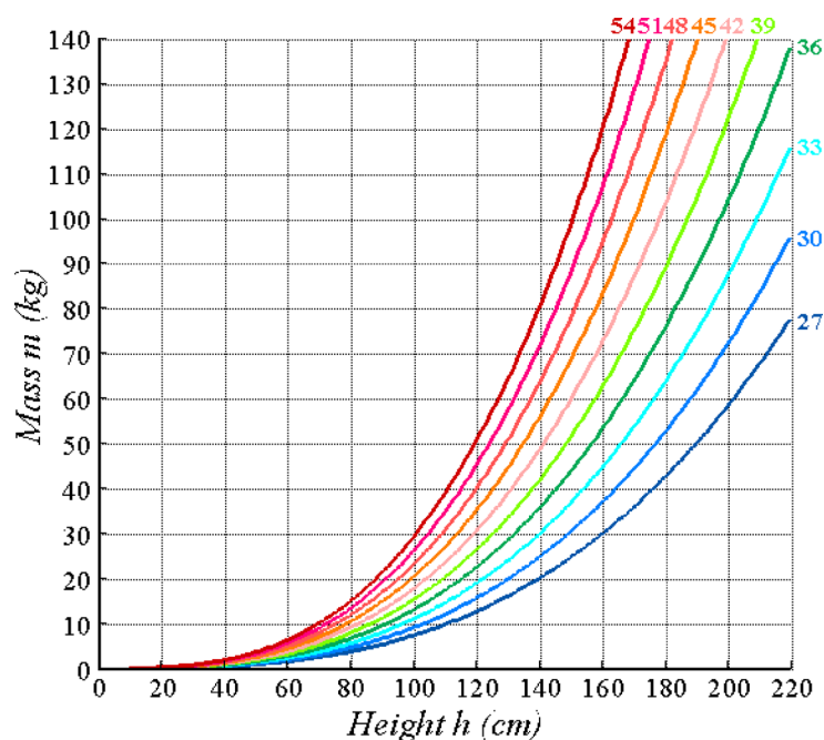
Fig. 4. Classification of anthropometric status levels according to 10 CBMI values. Interval between 33 and 39 normal levels with ideal average 36.
